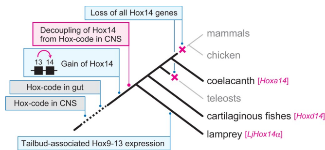
Fig. 4. A hypothesized evolutionary scenario of repertoires and roles of Hox14. Possession of Hox14 genes is indicated with the gene names beside the names of animal groups. The timings of possible losses of all Hox14 members are indicated with an "X."
