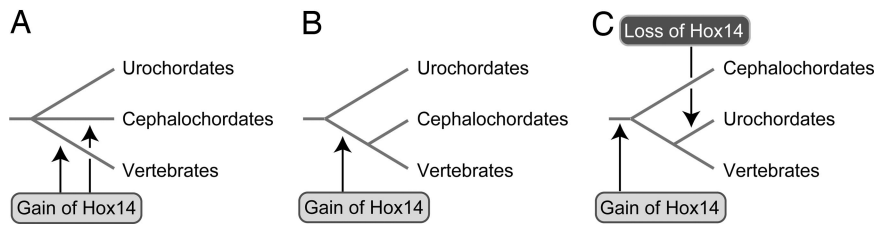
Fig. 1. Alternative scenarios for gains and a loss of Hox14. (A) Hox14 might have been gained independently in the cephalochordate and vertebrate lineages. (B) Under the assumption of traditional phylogenetic relationships between chordate subphyla (see ref. 15), if Hox14 of the amphioxus and vertebrates arose with a single event, the presence of Hox14 can be interpreted as a synapomorphy for the cephalochordate-vertebrate clade. (C) Under the phylogenetic relationships suggested by Delsuc et al. (15), if Hox14 of amphioxus and vertebrates are orthologous, we must assume a secondary loss of the Hox14 gene in the urochordate lineage.
