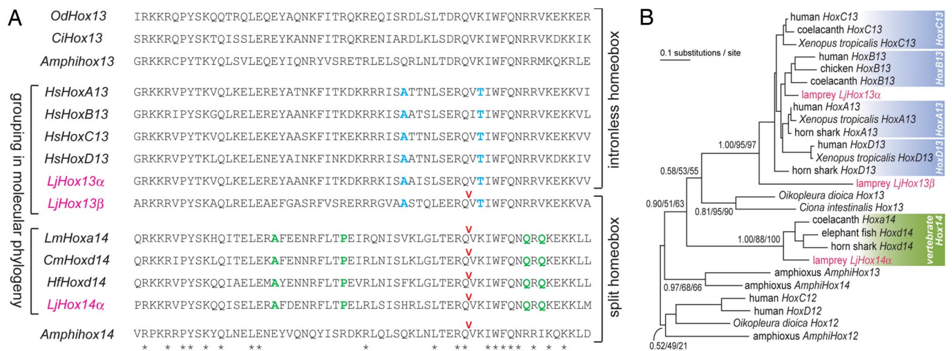
Fig. 2. Sequence comparison among Hox13/14 genes. (A) Amino acid sequences of the homeodomains of Hox13 and -14 genes. Amino acid residues that are conserved for all of these sequences are shown with asterisks below the alignment. Positions of introns are shown as “V” above the amino acid sequences. Amino acid residues specific to each paralogous group of Hox genes, based on comparison with paralogous group 1–12, are indicated with matching colors. Abbreviation of species names: Hs , Homo sapiens ; Lm , Latimeria menadoensis ; Lj , Lethenteron japonicum ; Hf , Heterodontus francisci ; Cm , Callorhynchus milii ; AmphiHox , amphioxus Hox . (B) A molecular phylogeny of chordate Hox13 and Hox14 genes. This tree was inferred with the ML method using amino acid sequences (58 aa) using Hox12 genes as an outgroup. The JTT+I+G 4 model was assumed ( \alpha = 0.37 ). Support for critical nodes are shown in the order, posterior probabilities of the Bayesian analysis, support values of ML analysis using quartet-puzzling, and bootstrap probabilities of the neighbor-joining tree inference with 1,000 iterations (17). Note that the clustering of vertebrate Hox13 genes and tunicate Hox13 genes is not strongly supported.
